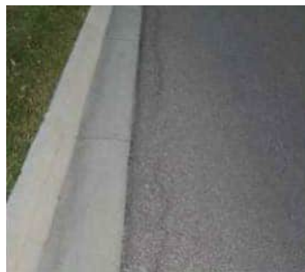
Figure 27 Low Edge Cracking PAVERTM Distress Identification Manual
